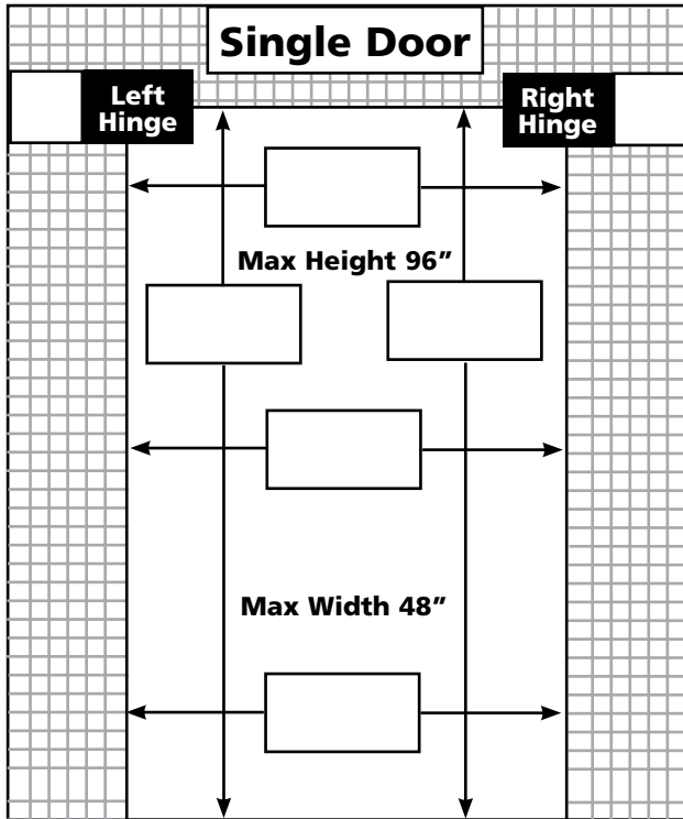
Opening dimensions in inches
