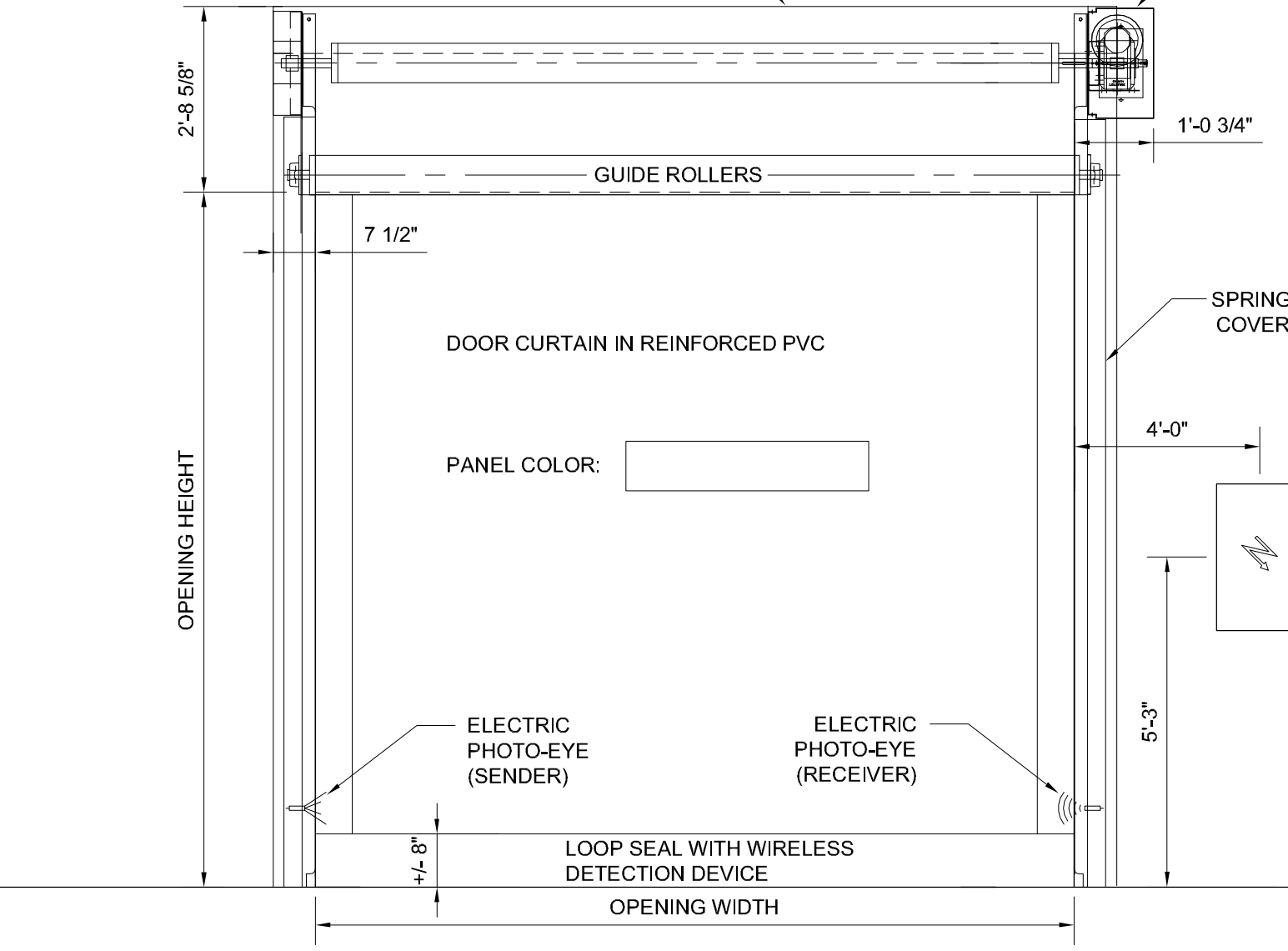
ELEVATION VIEW - FRONT
