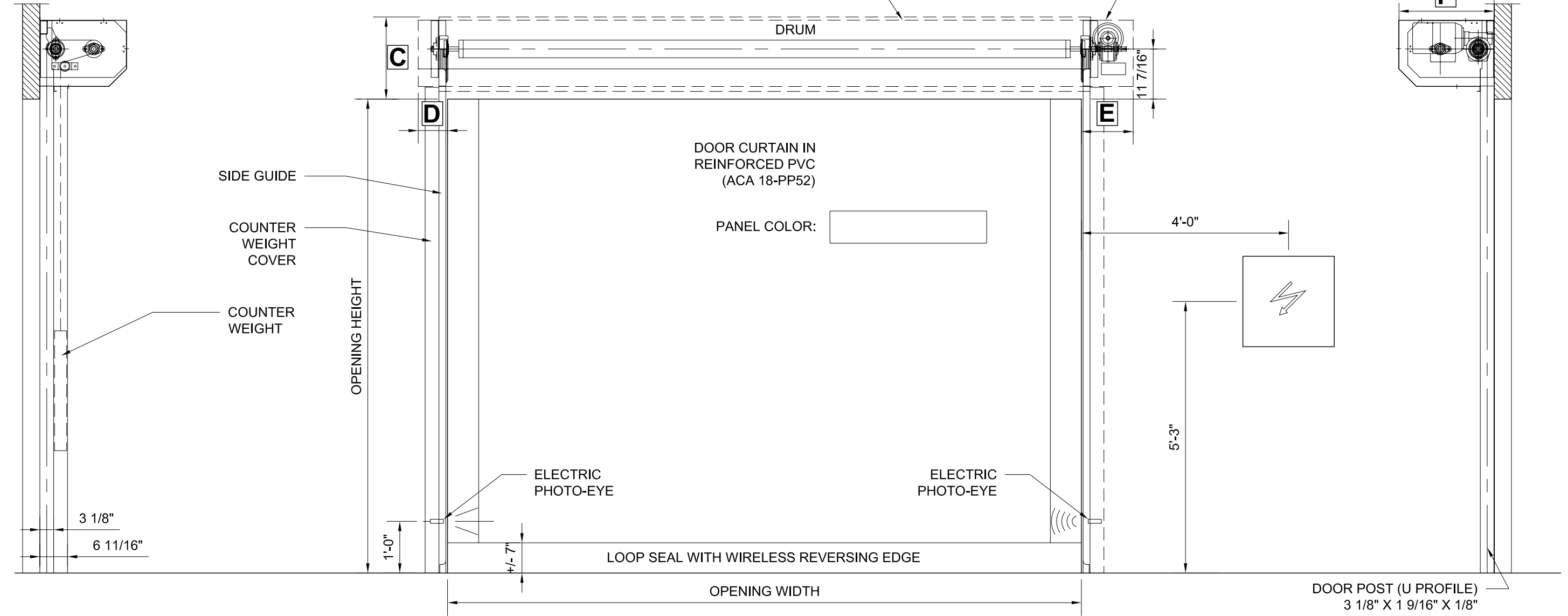
ELEVATION VIEW - LEFT
